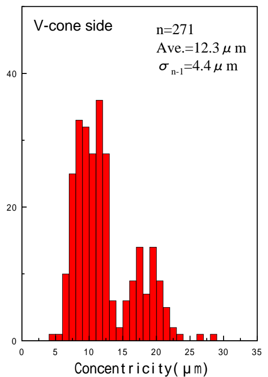
Fig.-Results of concentricity measurement Sample; Blank (after centerless grinding)
