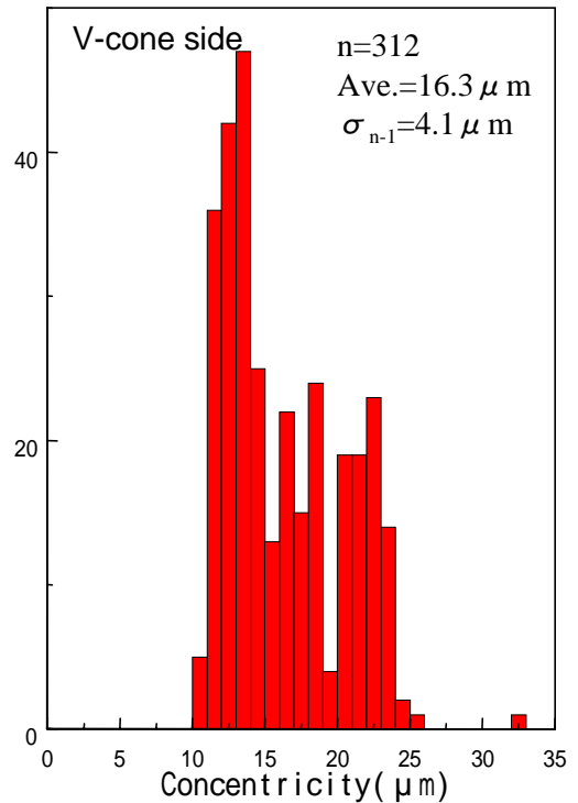
Fig.-Results of concentricity measurement Sample; Blank (before centerless grinding)
