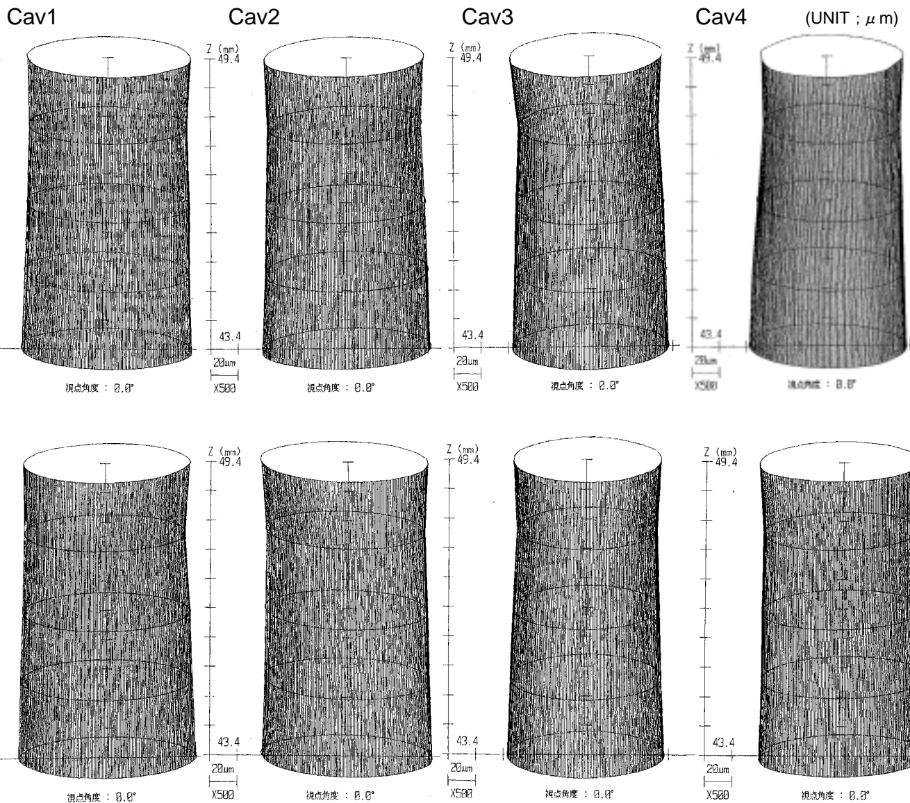
Fig.- Cylindricity of Outer Diameter
