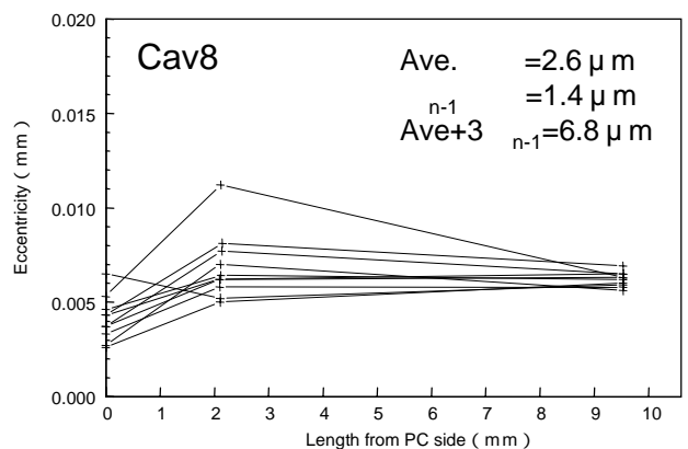
Fig.- Straightness of Micro-hole
